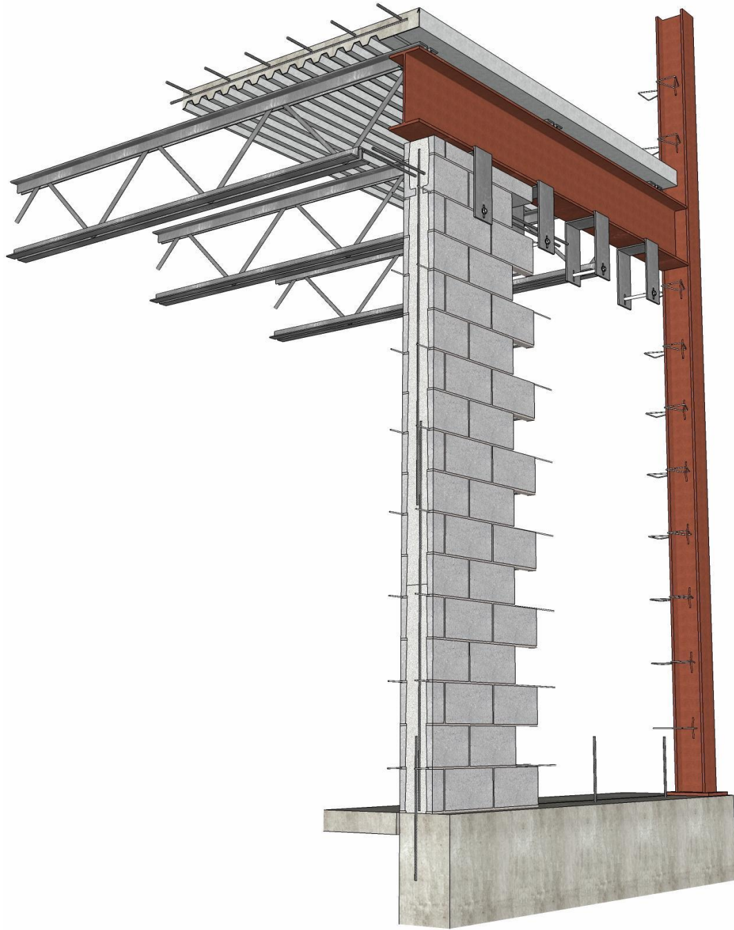
WALL SECTION HYBRID WALL SYSTEM DETAIL 02.120.0102 REV. 08/21/09
