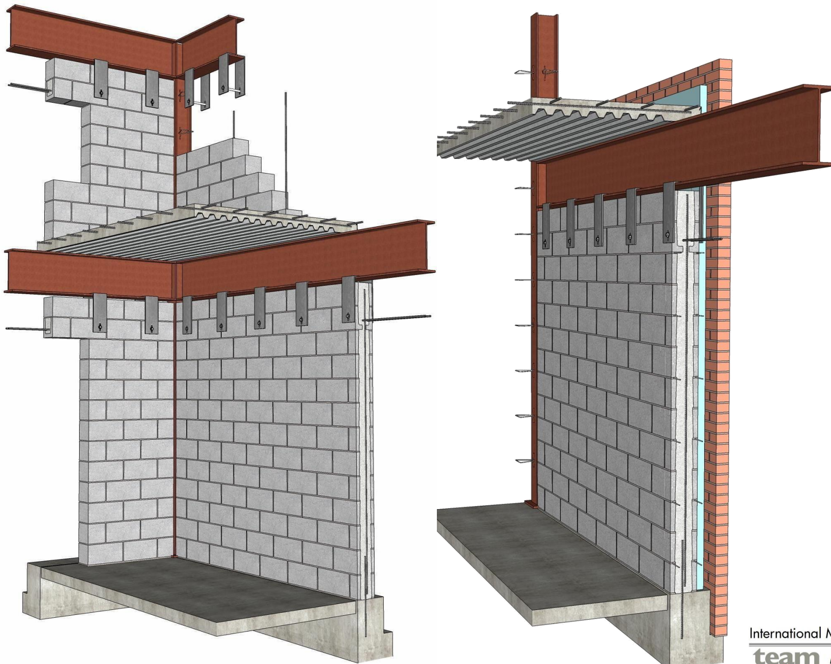
WALL SECTION HYBRID WALL SYSTEM DETAIL 02.120.0101 REV. 08/21/09
