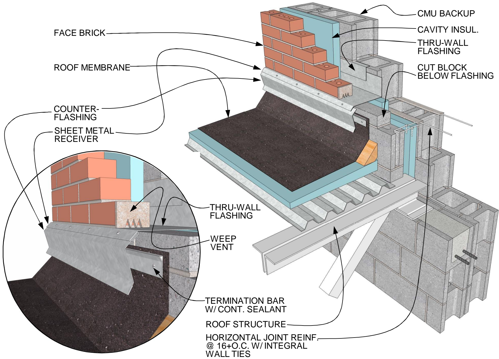
ROOF DETAIL HIGH WALL . LOW ROOF DETAIL 01.030.0751 REV. 11/6/07
