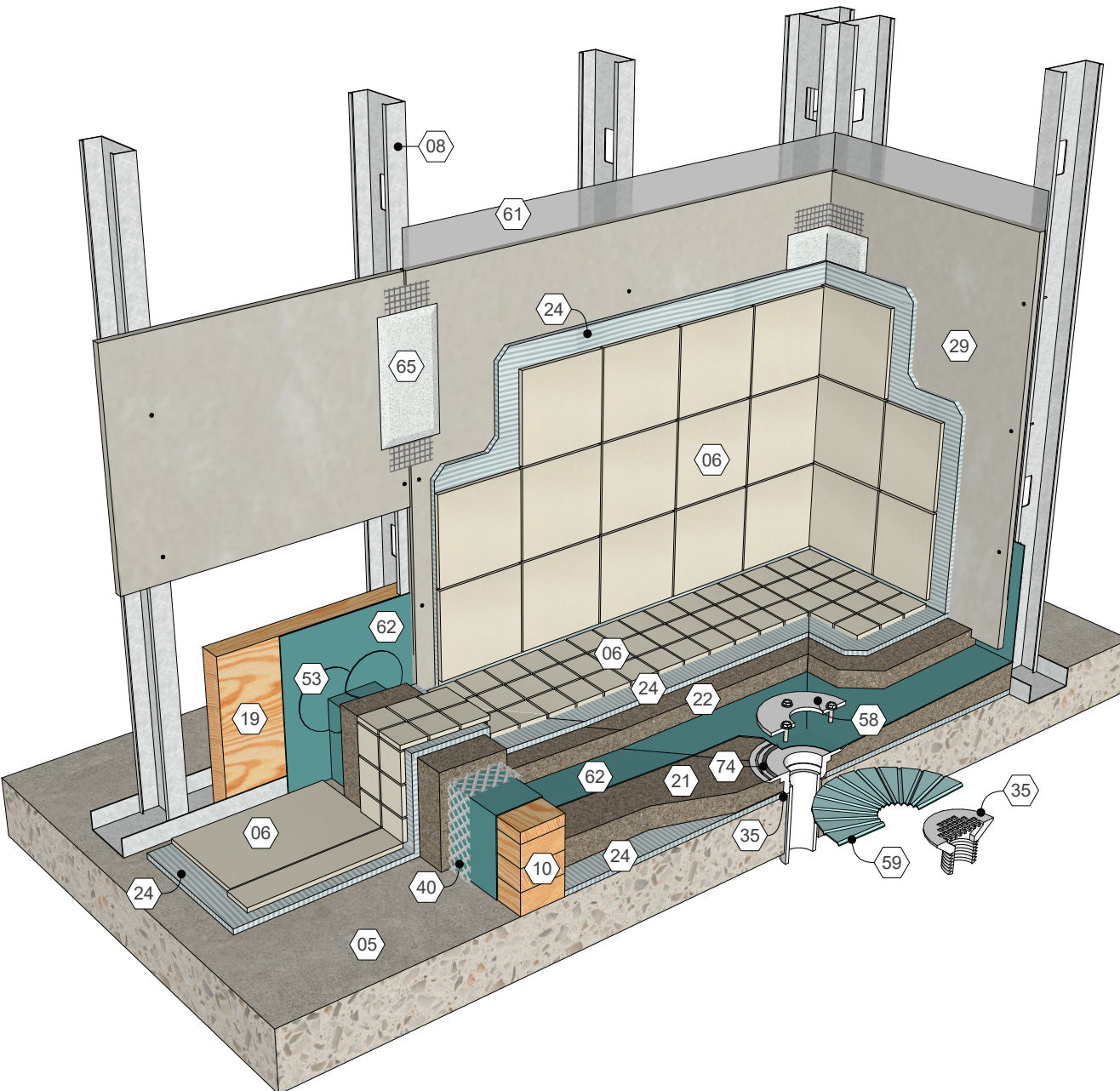
Tile shower assembly | Metal studs, CBU backing, mortar bed floor, two-stage drain, ceramic tile Detail 06.110.0415
