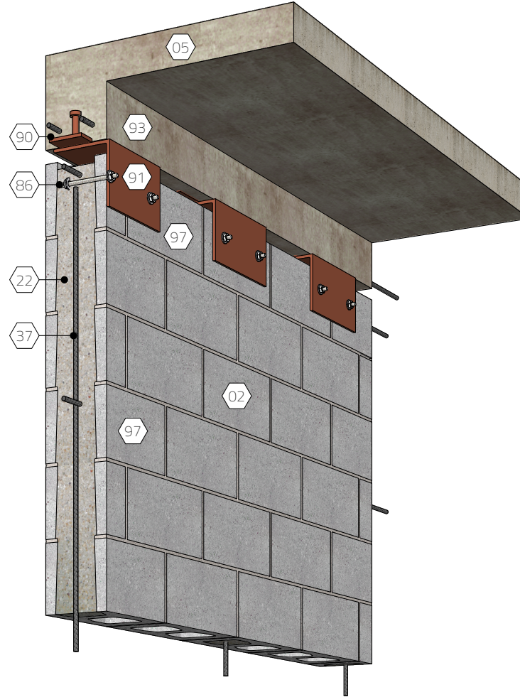
Masonry restraint at concrete beam
