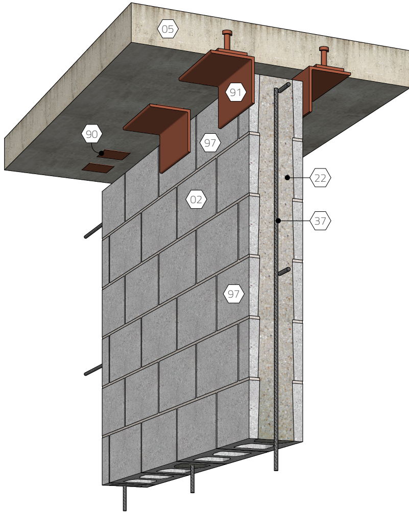
Masonry restraint at concrete slab
