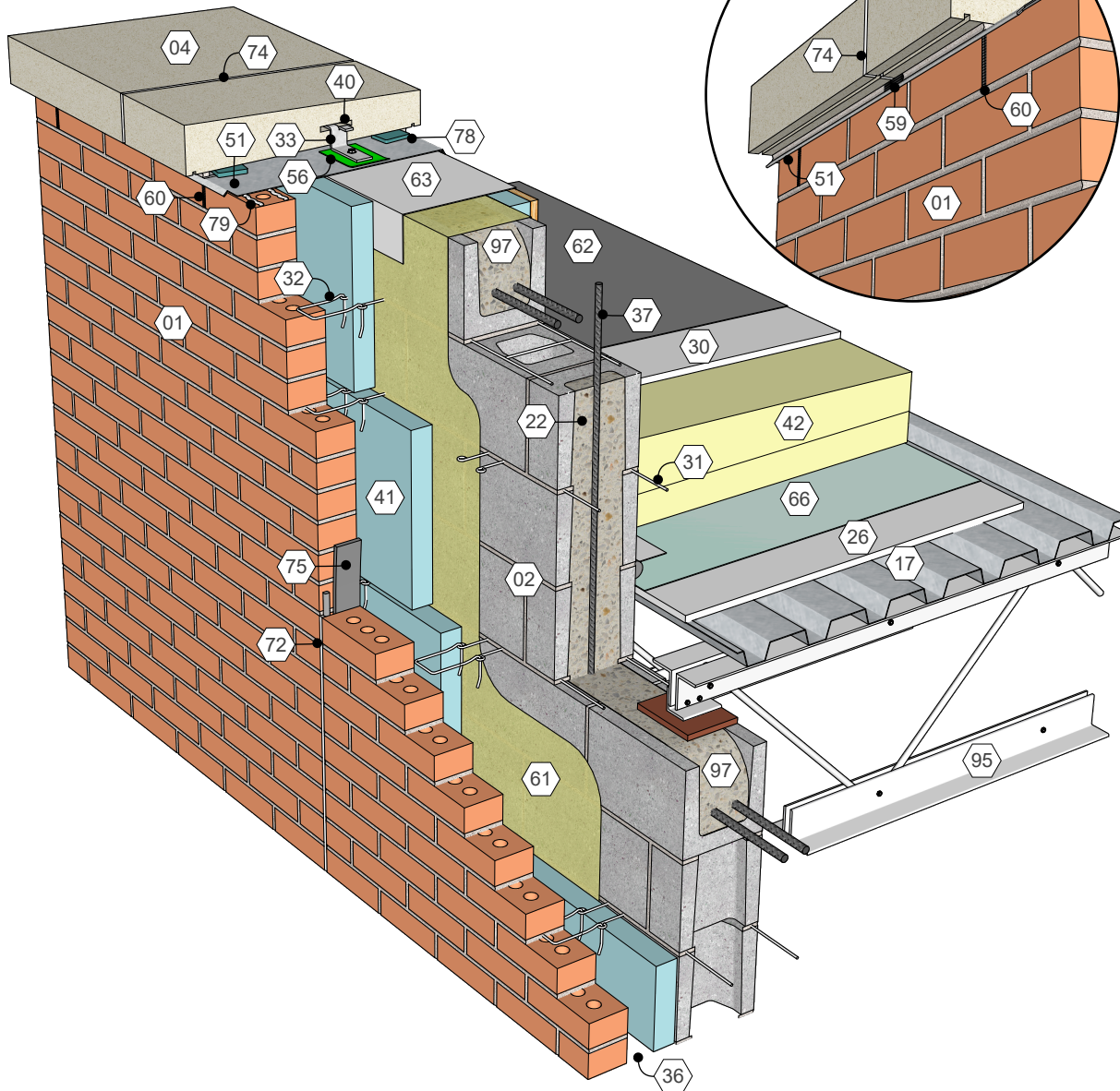
Top of Wall, Outside View | Anchored Brick veneer, CMU Backing Detail 01.030.0901 Rev. 04/14/21
