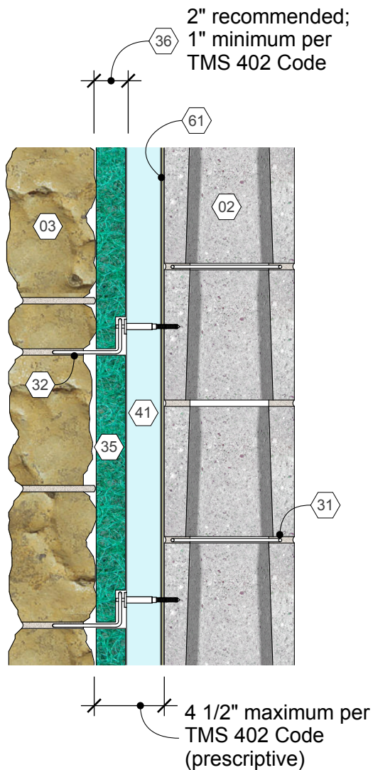
Stone Veneer, CMU Backup Detail 03.030.0201 Rev. 7/28/16
