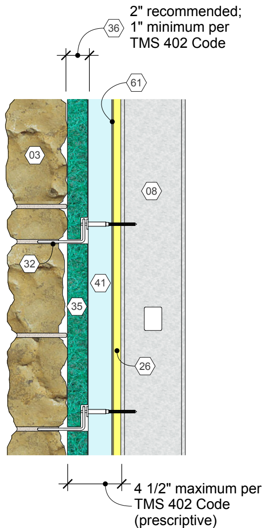
Stone Veneer, Steel Stud Backup Detail 03.040.0201 Rev. 7/28/16
