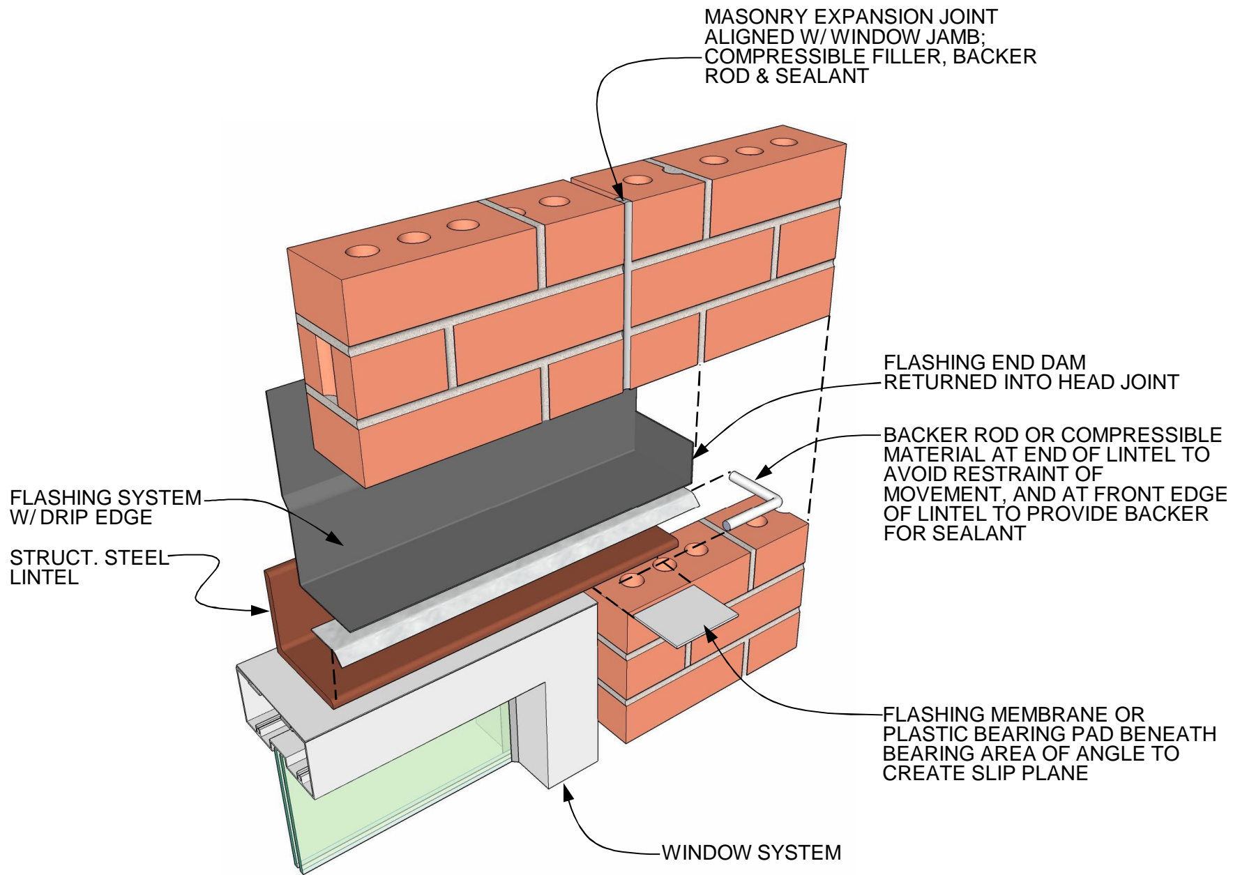
EXPANSION JOINT AT WINDOW DETAIL 01.030.1321 REV. 08/09/09
