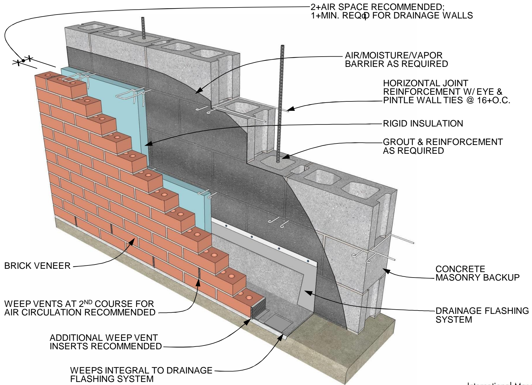
BASE OF WALL DETAIL DRAINAGE FLASHING DETAIL 01.030.0304 REV. 09/25/09
