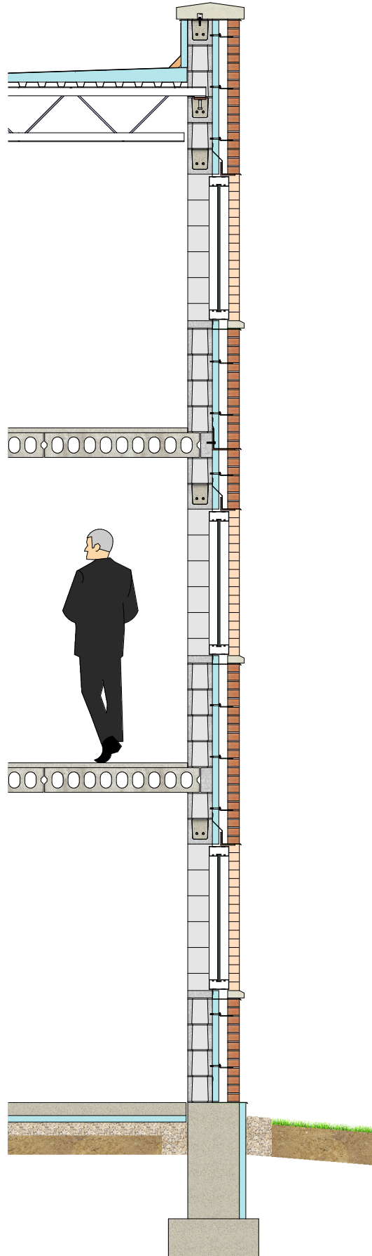
Conceptual Wall Section, Brick veneer, CMU backup Detail 01.030.0101 Rev. 09/25/17
